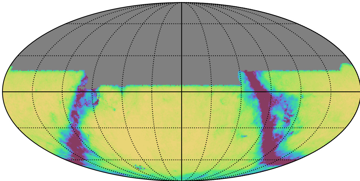
noroll_mjdp365_v3.4_10yrs All sky u band: Exgal_CoaddM5
