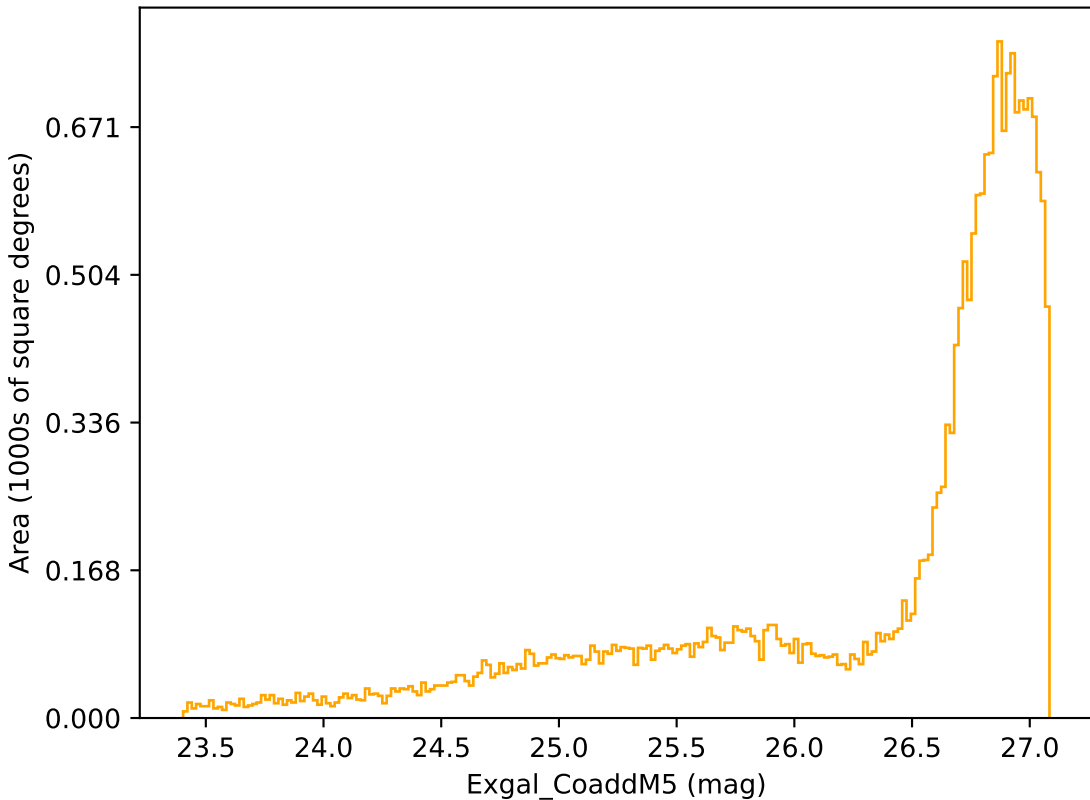
noroll_mjdp365_v3.4_10yrs All sky r band: Exgal_CoaddM5
