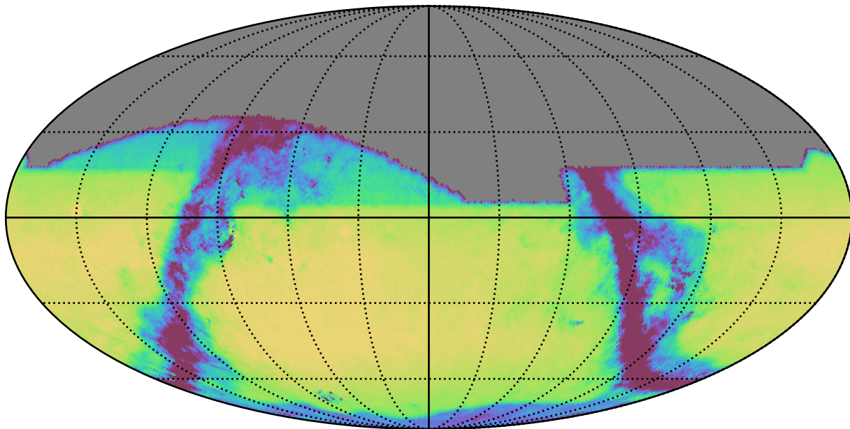
noroll_mjdp365_v3.4_10yrs All sky i band: Exgal_CoaddM5
