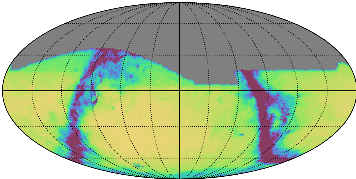
noroll_mjdp365_v3.4_10yrs All sky g band: Exgal_CoaddM5
