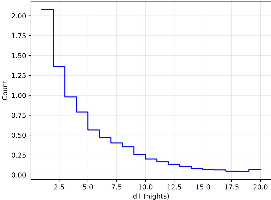
noroll_mjdp365_v3.4_10yrs WFD all bands: DeltaNight Histogram
