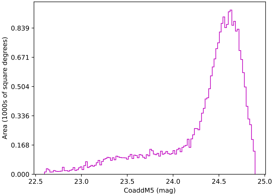
noroll_mjdp365_v3.4_10yrs Yr 3-4 z band: CoaddM5
