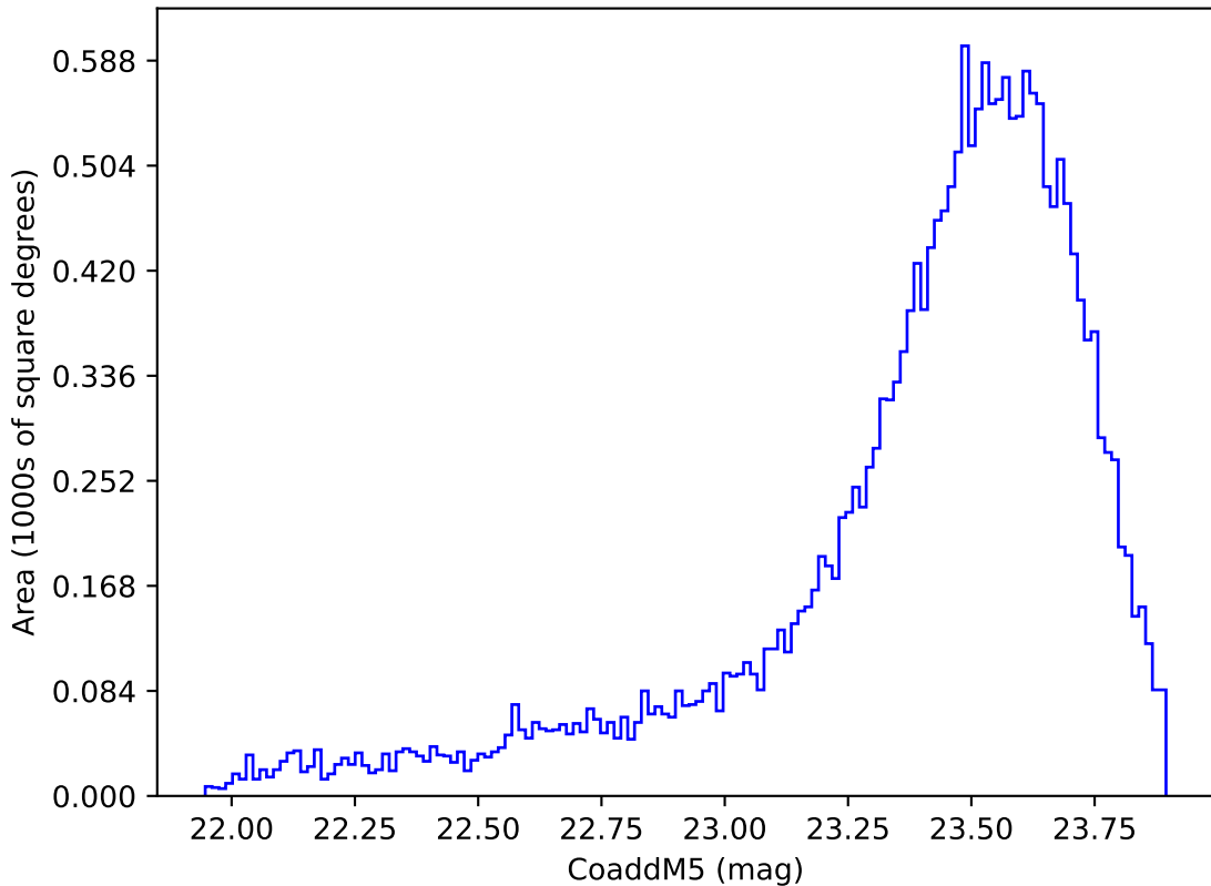
noroll_mjdp365_v3.4_10yrs Yr 3-4 y band: CoaddM5
