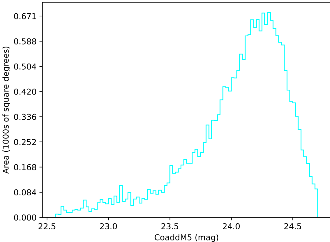
noroll_mjdp365_v3.4_10yrs Yr 3-4 u band: CoaddM5
