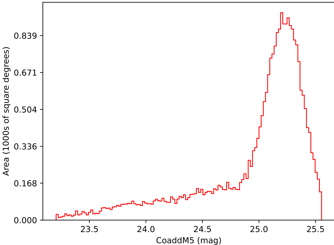
noroll_mjdp365_v3.4_10yrs Yr 3-4 i band: CoaddM5
