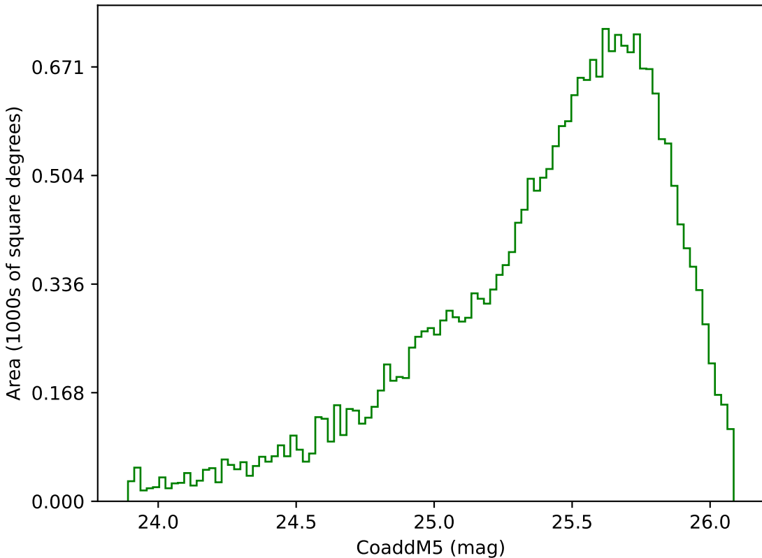
noroll_mjdp365_v3.4_10yrs Yr 3-4 g band: CoaddM5
