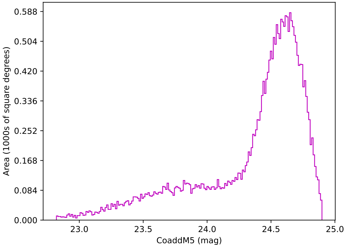
noroll_mjdp365_v3.4_10yrs Yr 1 z band: CoaddM5
