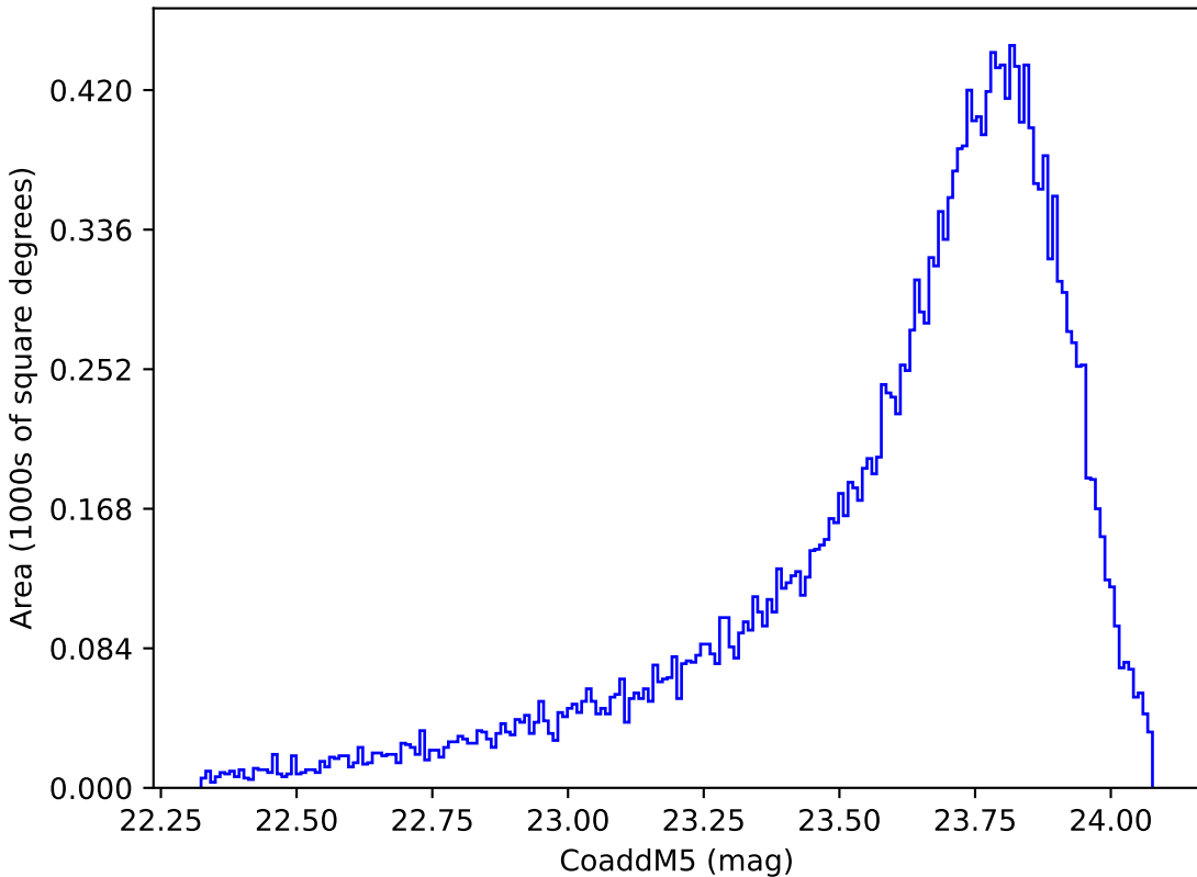
noroll_mjdp365_v3.4_10yrs Yr 1 y band: CoaddM5
