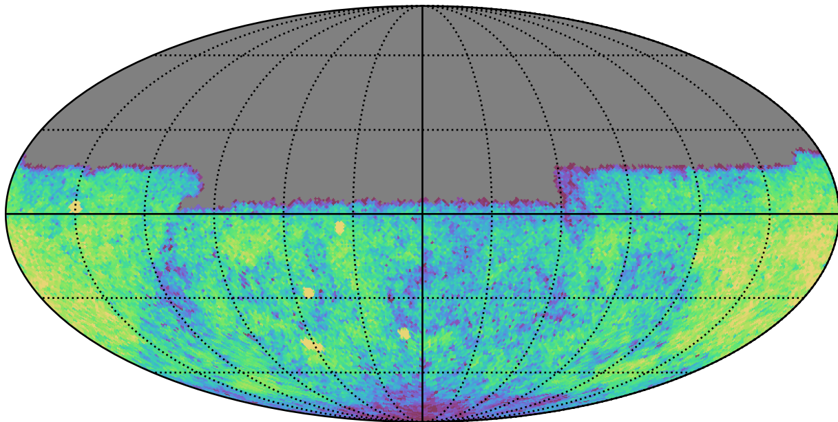
noroll_mjdp365_v3.4_10yrs Yr 1 u band: CoaddM5
