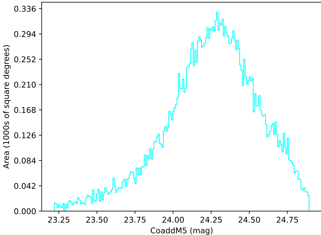
noroll_mjdp365_v3.4_10yrs Yr 1 u band: CoaddM5
