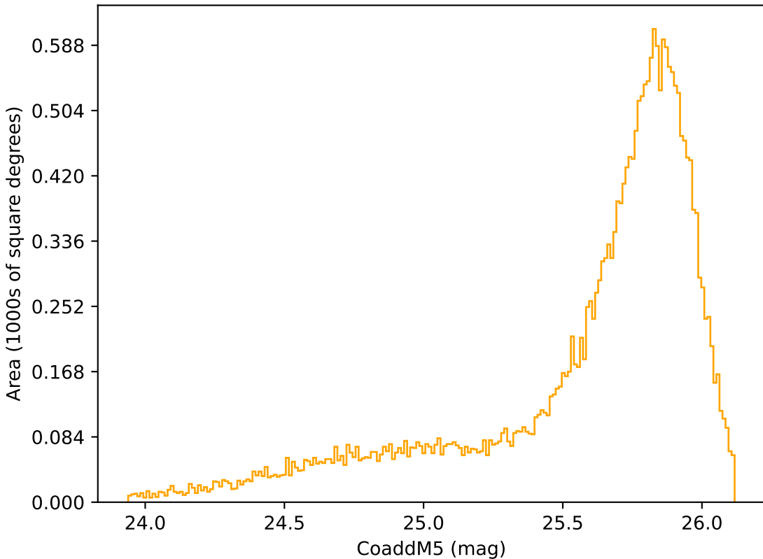
noroll_mjdp365_v3.4_10yrs Yr 1 r band: CoaddM5
