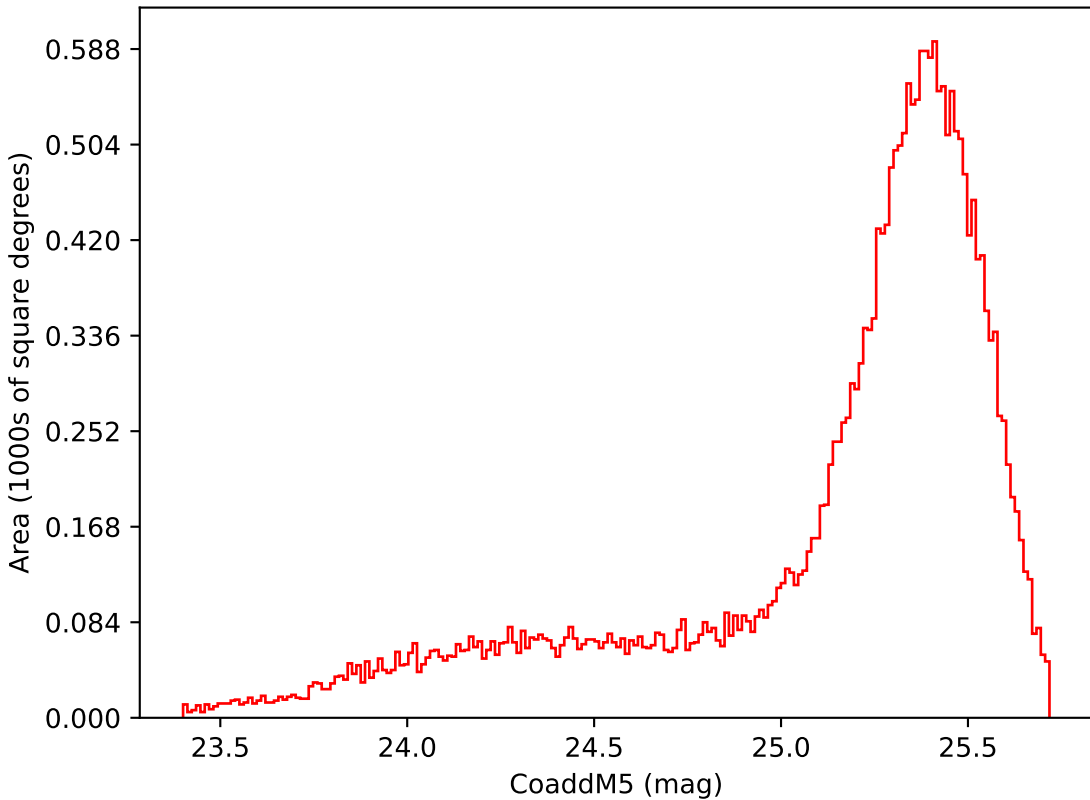
noroll_mjdp365_v3.4_10yrs Yr 1 i band: CoaddM5
