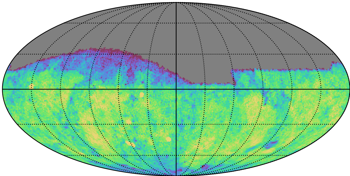
noroll_mjdp365_v3.4_10yrs Yr 1 g band: CoaddM5
