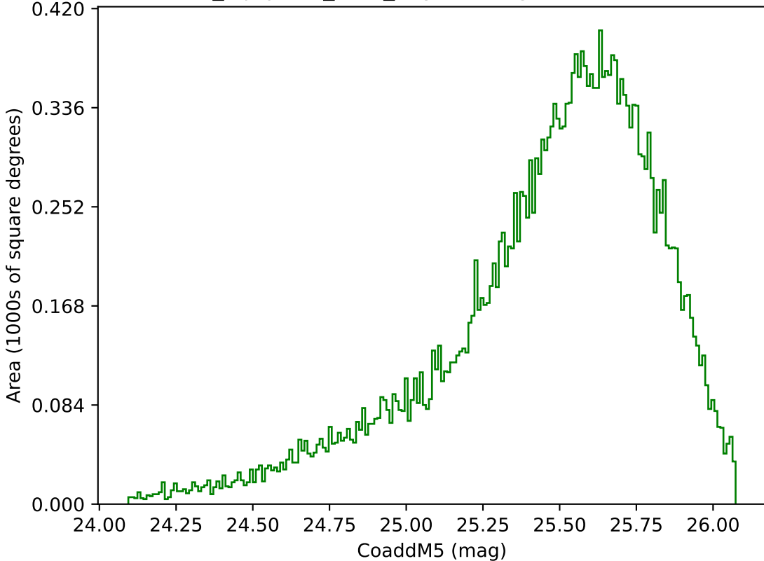
noroll_mjdp365_v3.4_10yrs Yr 1 g band: CoaddM5
