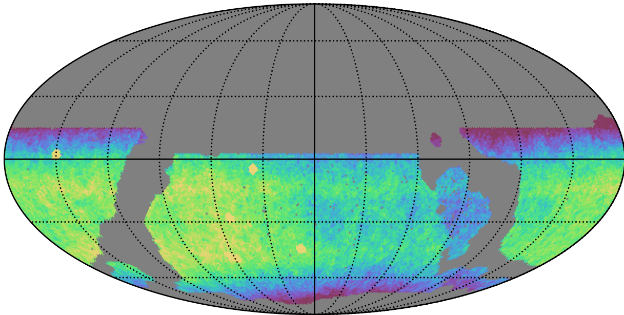
noroll_mjdp365_v3.4_10yrs WFD z band: CoaddM5
