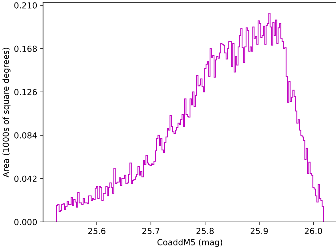
noroll_mjdp365_v3.4_10yrs WFD z band: CoaddM5
