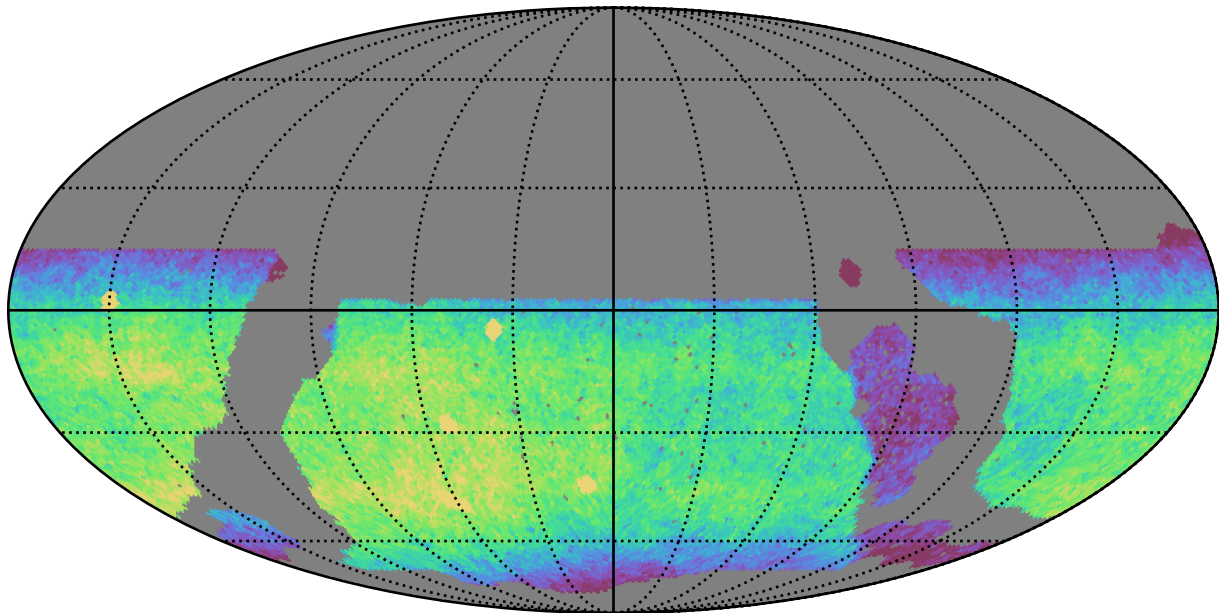
noroll_mjdp365_v3.4_10yrs WFD y band: CoaddM5
