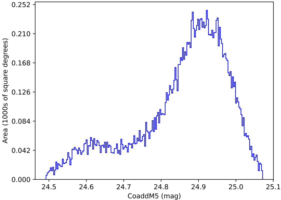
noroll_mjdp365_v3.4_10yrs WFD y band: CoaddM5
