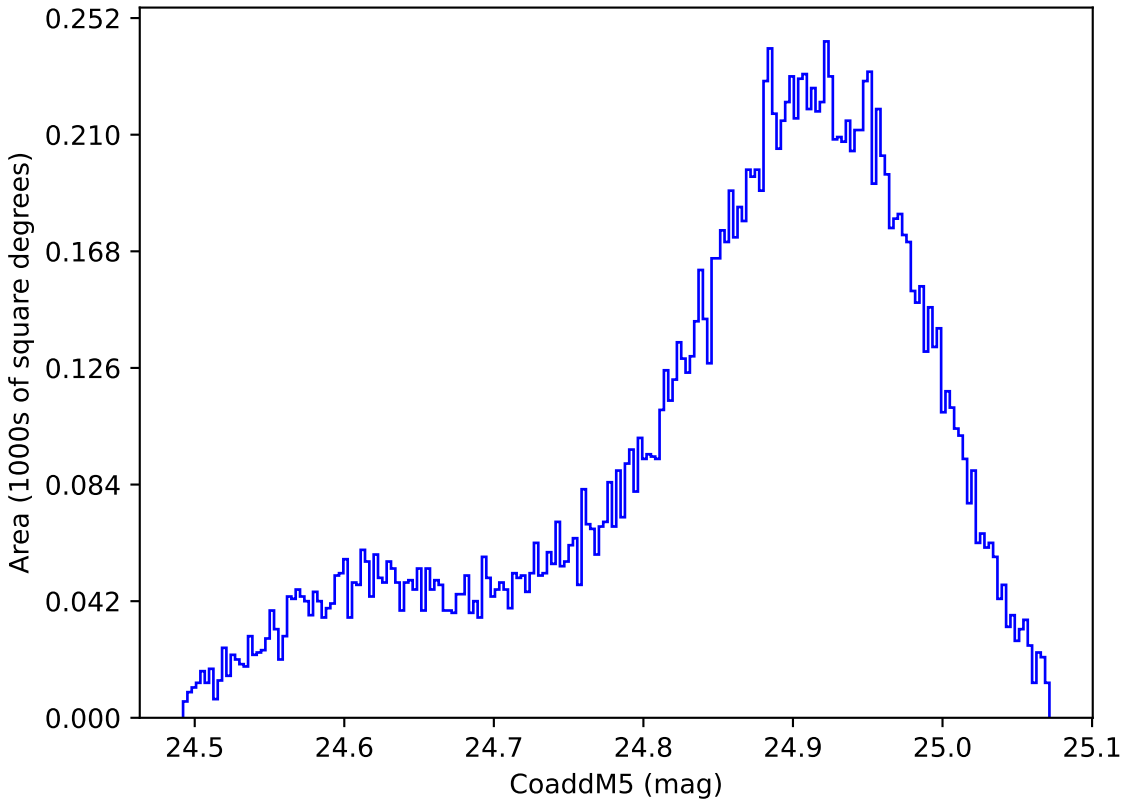
noroll_mjdp365_v3.4_10yrs WFD y band: CoaddM5
