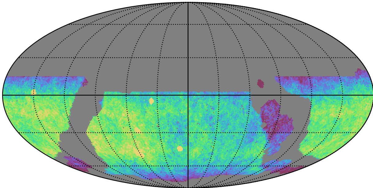
noroll_mjdp365_v3.4_10yrs WFD u band: CoaddM5
