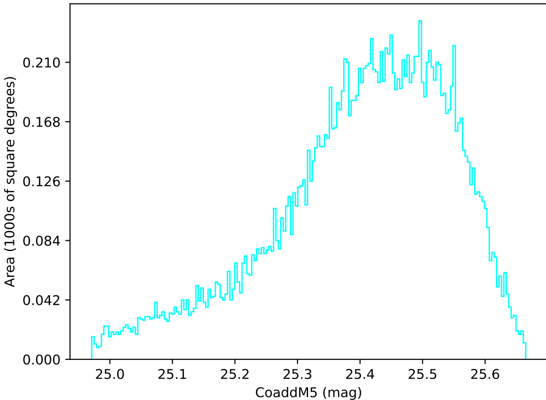
noroll_mjdp365_v3.4_10yrs WFD u band: CoaddM5
