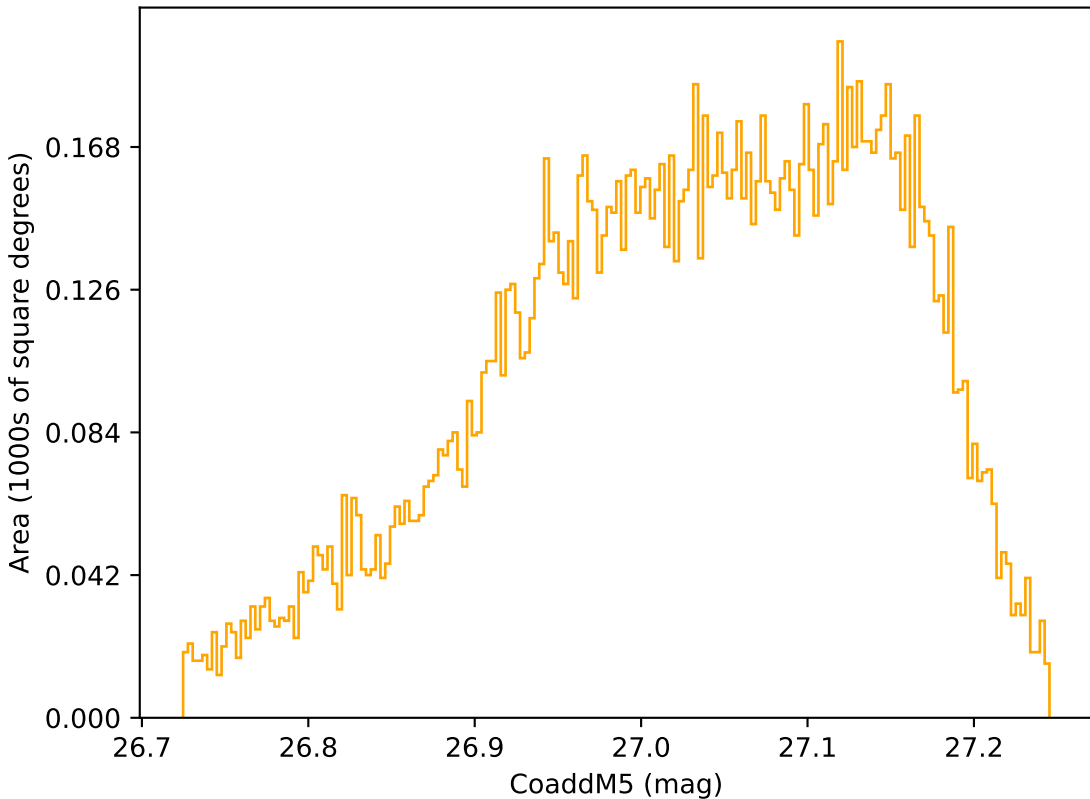
noroll_mjdp365_v3.4_10yrs WFD r band: CoaddM5
