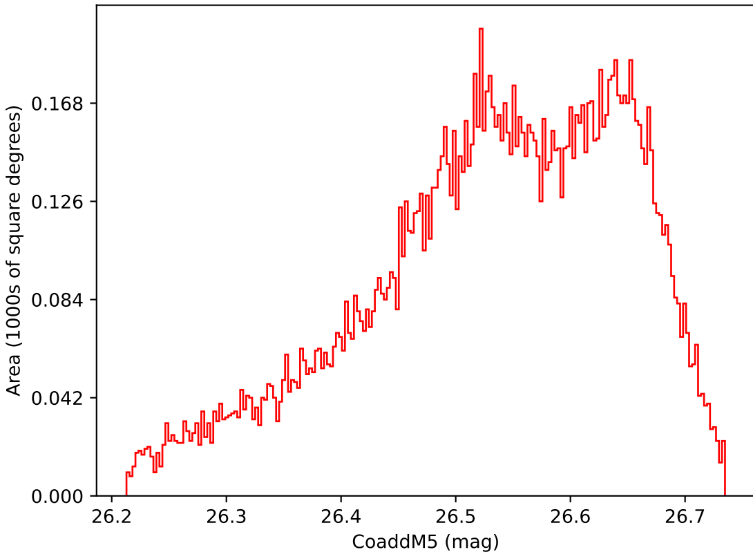
noroll_mjdp365_v3.4_10yrs WFD i band: CoaddM5
