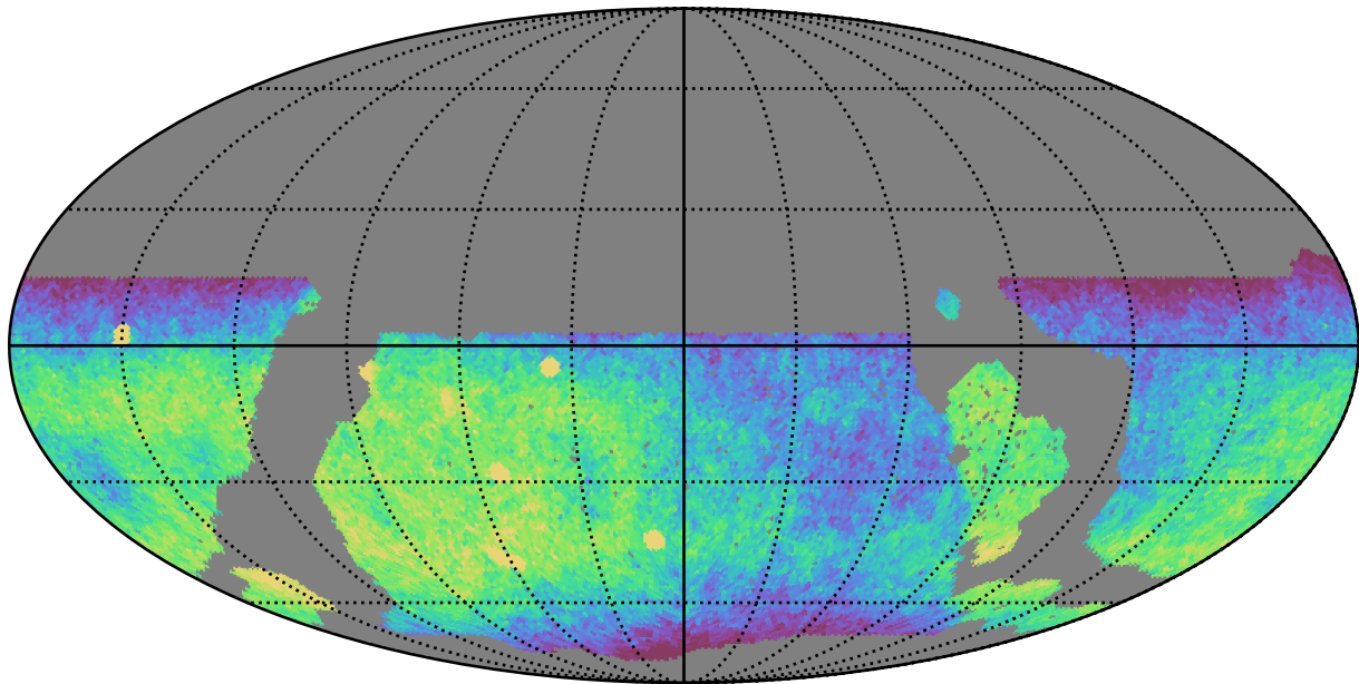
noroll_mjdp365_v3.4_10yrs WFD g band: CoaddM5
