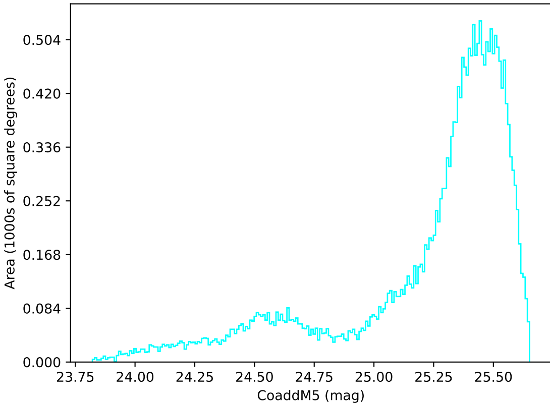
noroll_mjdp365_v3.4_10yrs All sky u band: CoaddM5
