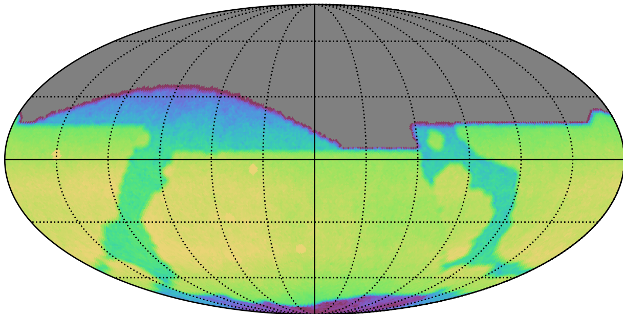
noroll_mjdp365_v3.4_10yrs All sky r band: CoaddM5
