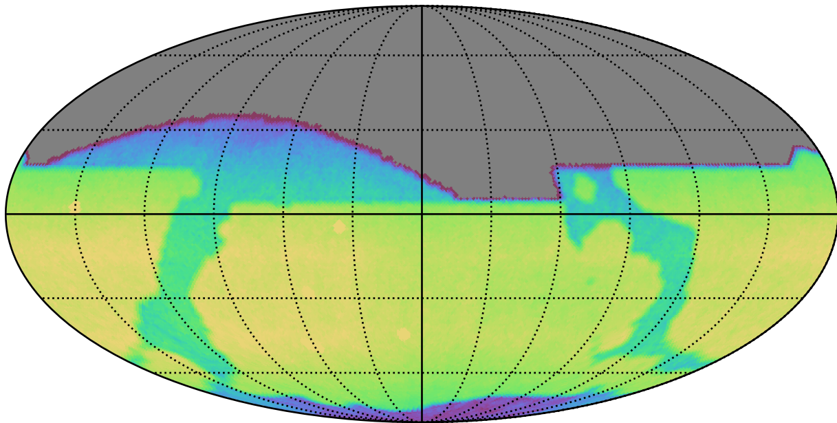
noroll_mjdp365_v3.4_10yrs All sky i band: CoaddM5
