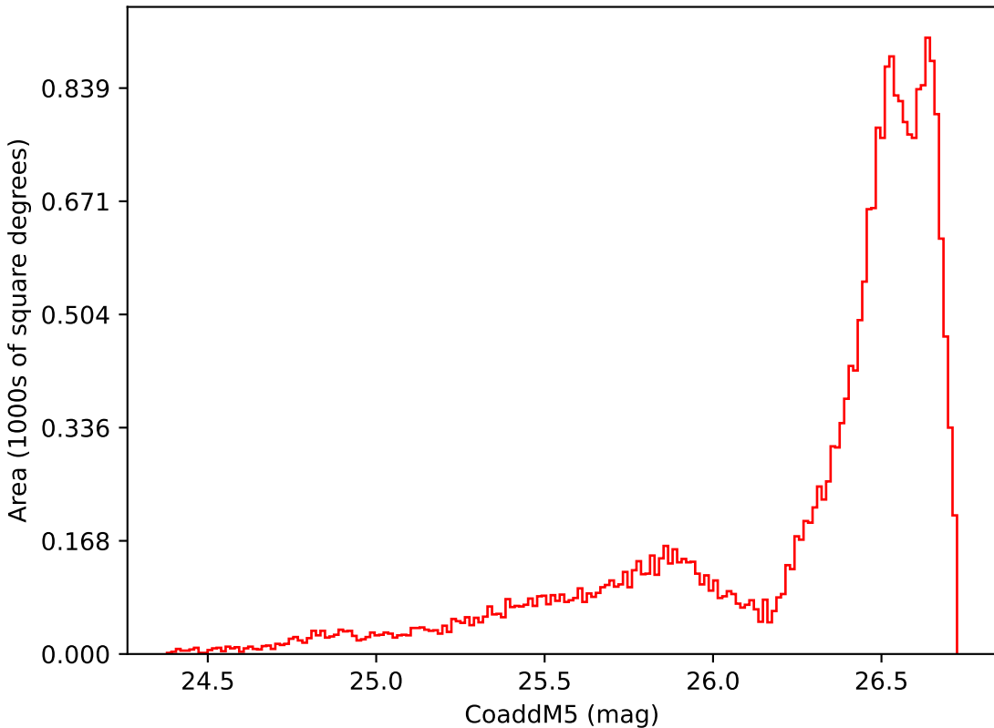
noroll_mjdp365_v3.4_10yrs All sky i band: CoaddM5
