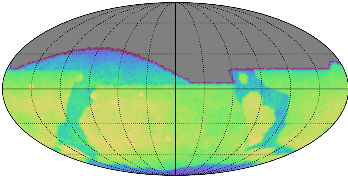
noroll_mjdp365_v3.4_10yrs All sky g band: CoaddM5
