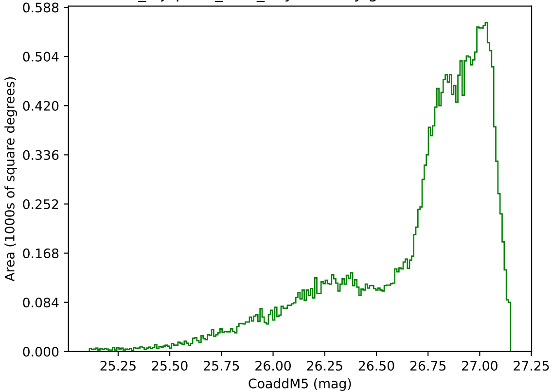
noroll_mjdp365_v3.4_10yrs All sky g band: CoaddM5
