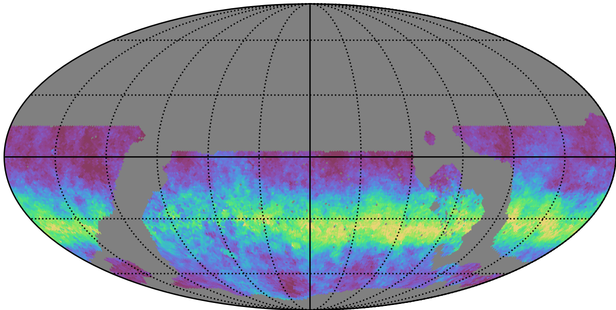
noroll_mjdp365_v3.4_10yrs WFD u band: AngleRms rotSkyPos
