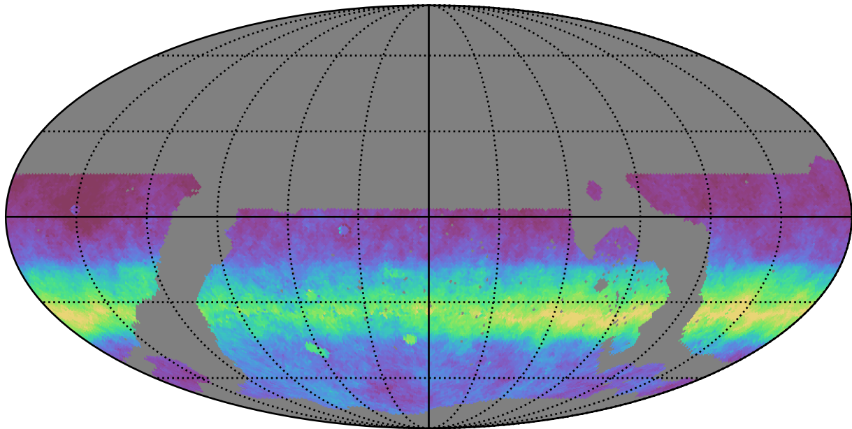
noroll_mjdp365_v3.4_10yrs WFD r band: AngleRms rotSkyPos
