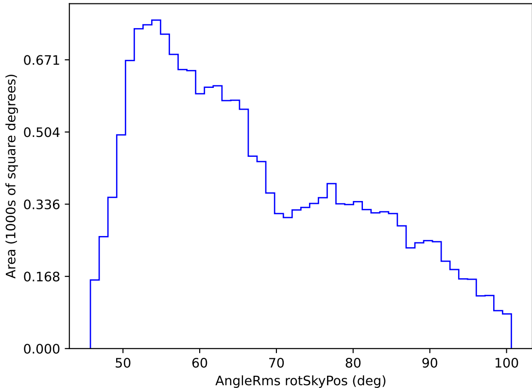
noroll_mjdp365_v3.4_10yrs WFD r band: AngleRms rotSkyPos
