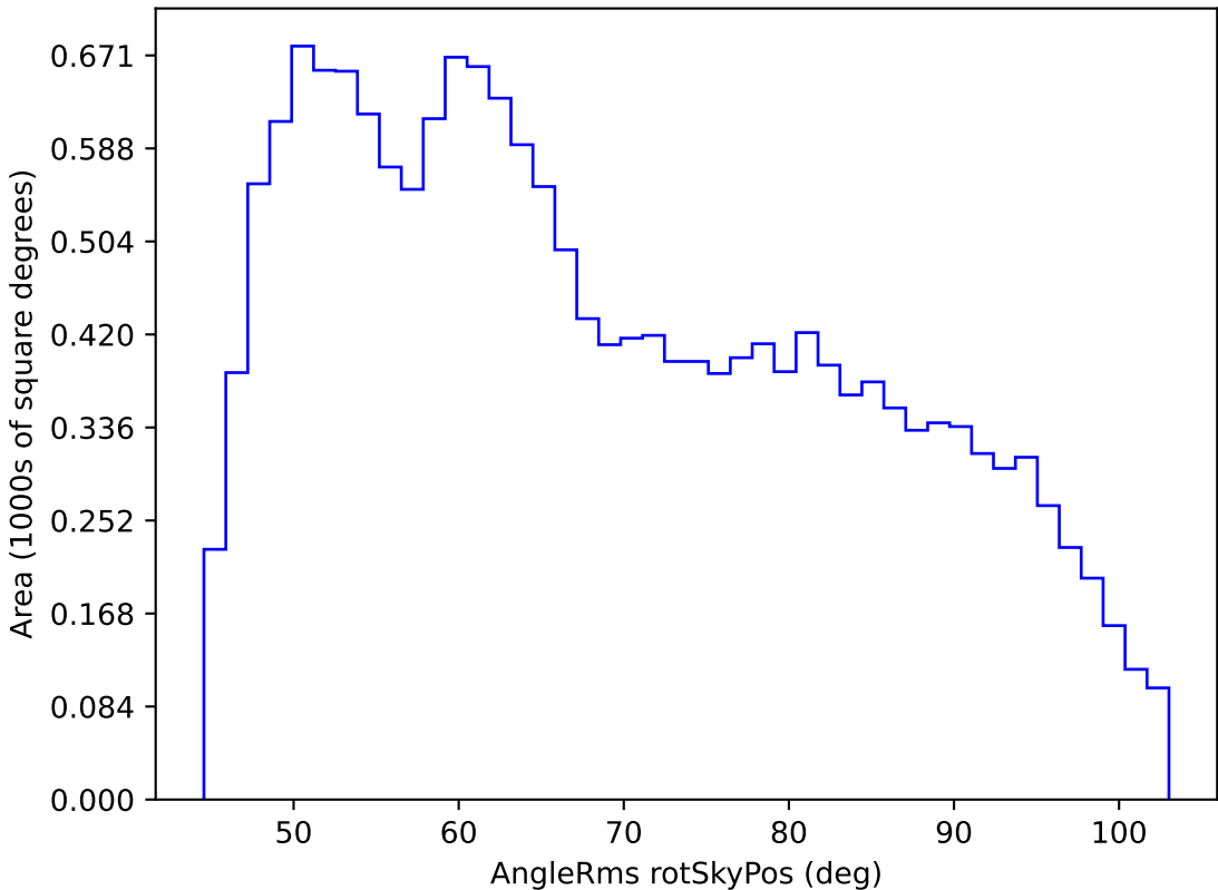
noroll_mjdp365_v3.4_10yrs WFD g band: AngleRms rotSkyPos
