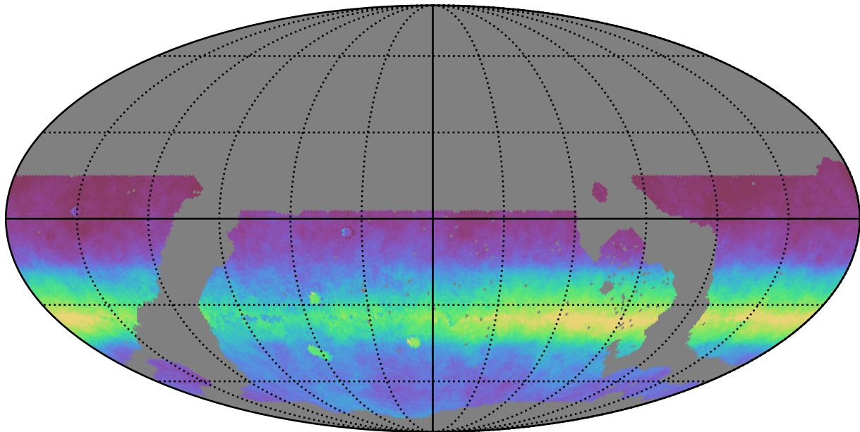
noroll_mjdp365_v3.4_10yrs WFD all bands: AngleRms rotSkyPos
