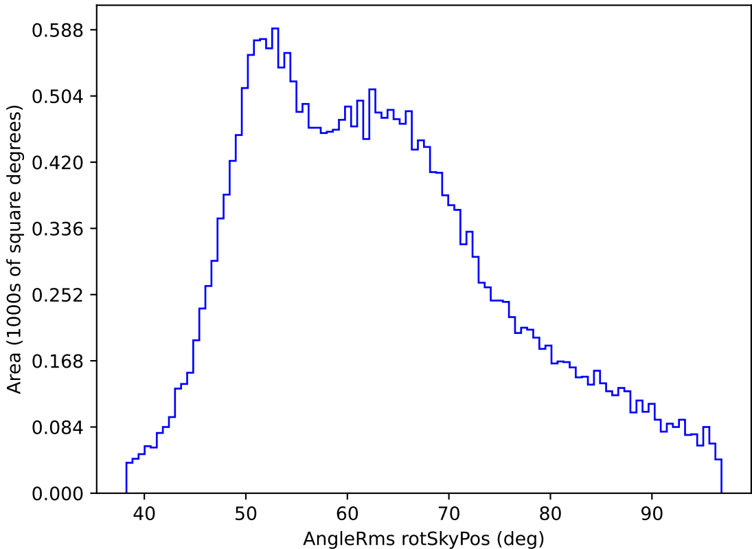
noroll_mjdp365_v3.4_10yrs All sky z band: AngleRms rotSkyPos
