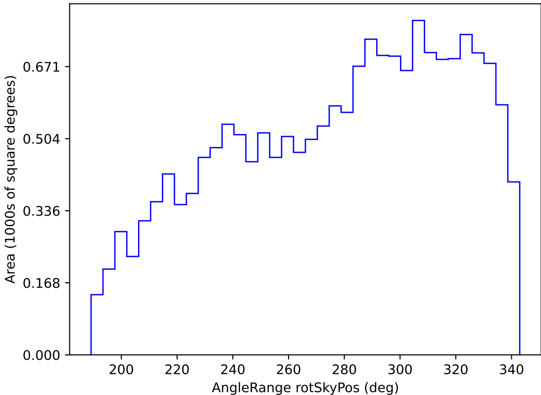
noroll_mjdp365_v3.4_10yrs WFD z band: AngleRange rotSkyPos
