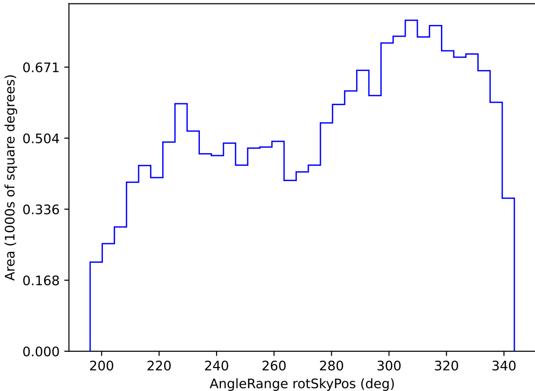
noroll_mjdp365_v3.4_10yrs WFD r band: AngleRange rotSkyPos
