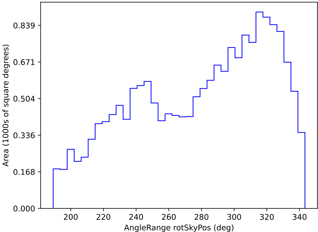
noroll_mjdp365_v3.4_10yrs WFD i band: AngleRange rotSkyPos
