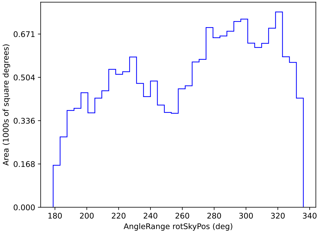
noroll_mjdp365_v3.4_10yrs WFD g band: AngleRange rotSkyPos
