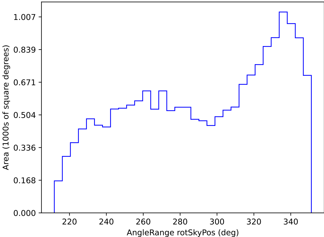
noroll_mjdp365_v3.4_10yrs WFD all bands: AngleRange rotSkyPos
