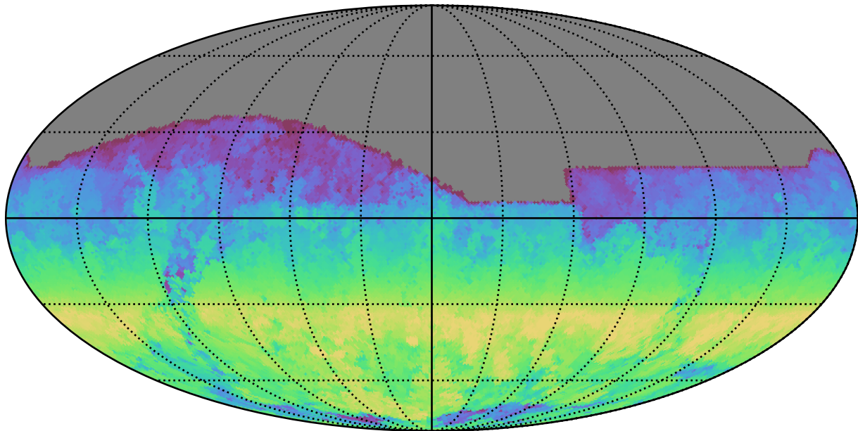
noroll_mjdp365_v3.4_10yrs All sky z band: AngleRange rotSkyPos
