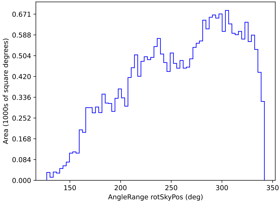
noroll_mjdp365_v3.4_10yrs All sky z band: AngleRange rotSkyPos
