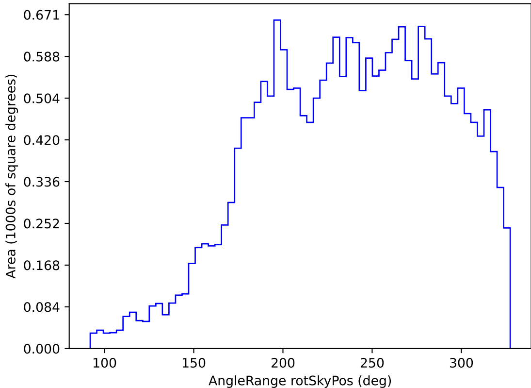
noroll_mjdp365_v3.4_10yrs All sky u band: AngleRange rotSkyPos
