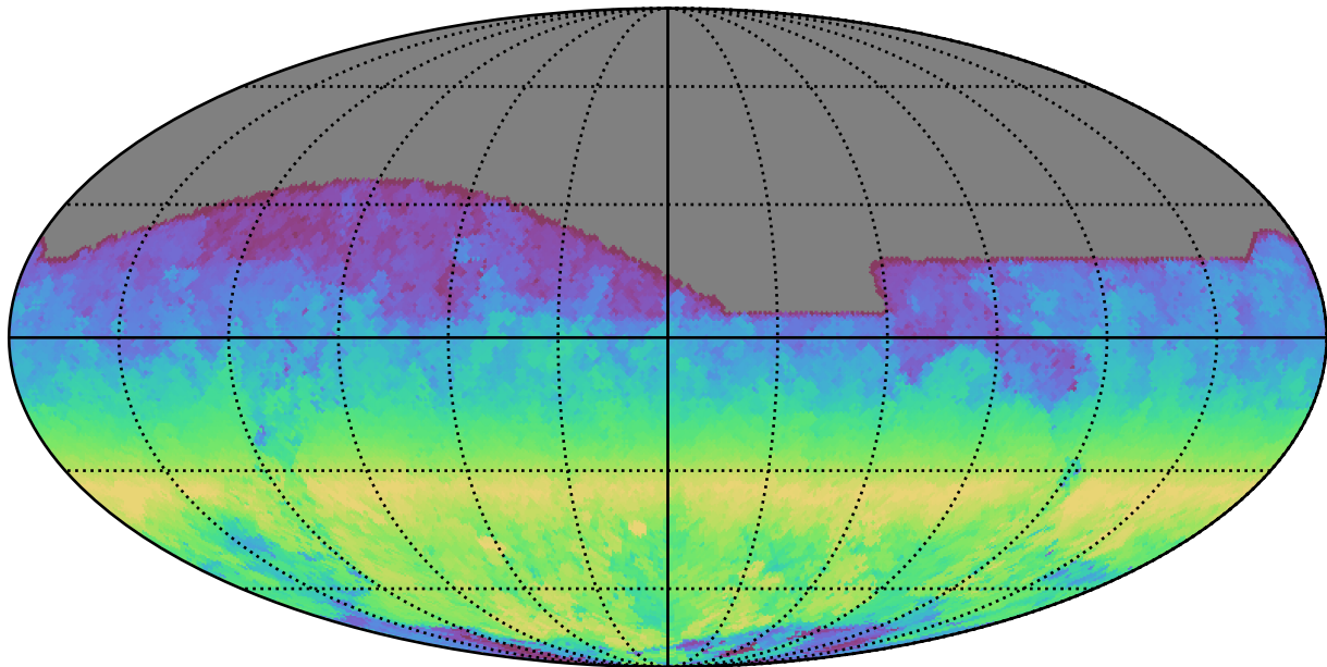
noroll_mjdp365_v3.4_10yrs All sky r band: AngleRange rotSkyPos
