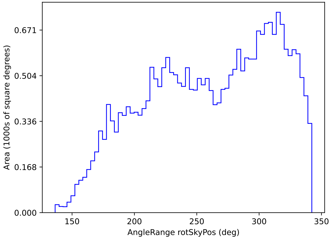
noroll_mjdp365_v3.4_10yrs All sky r band: AngleRange rotSkyPos
