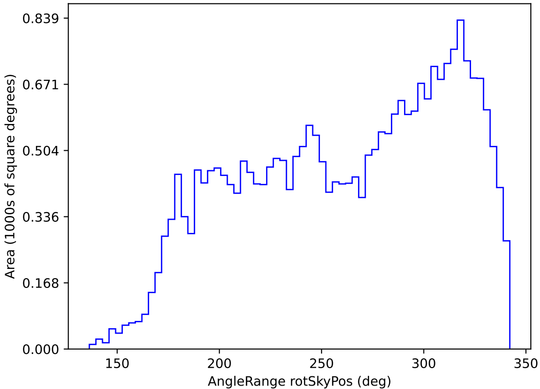
noroll_mjdp365_v3.4_10yrs All sky i band: AngleRange rotSkyPos
